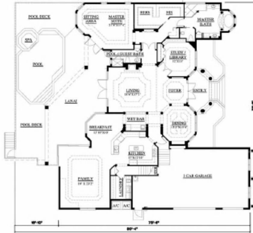
1st Floor
