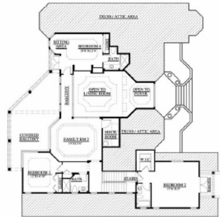
2nd Floor
